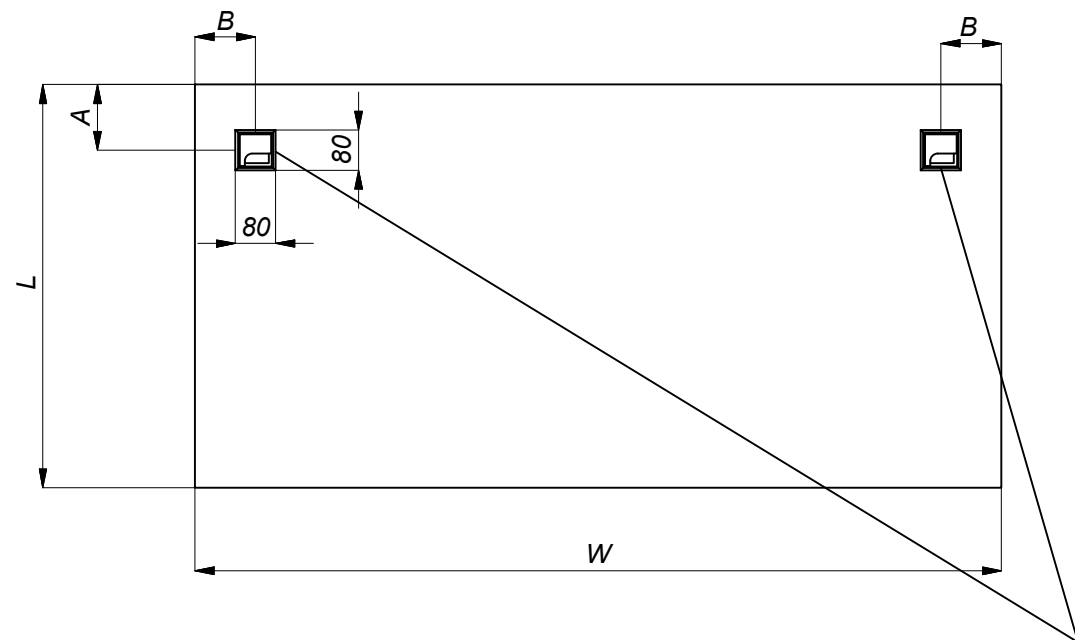
Set of Aluminium Cable Covers (Optional)
